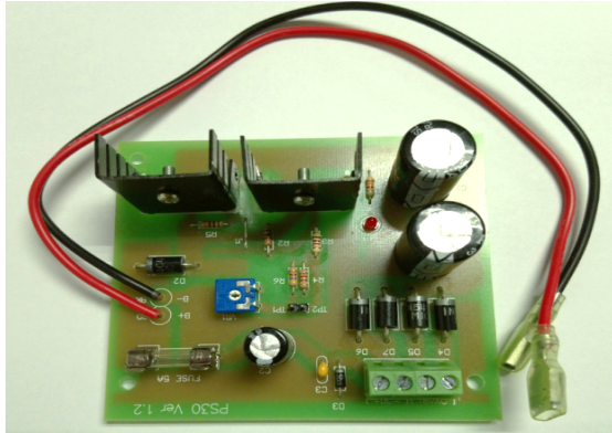
Linear Power Supply PCB
