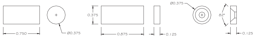
ALTERNATE RARE EARTH MAGNETS
